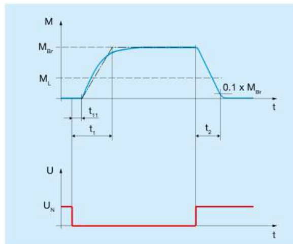
Diagram 4: Torque-Time Diagram
