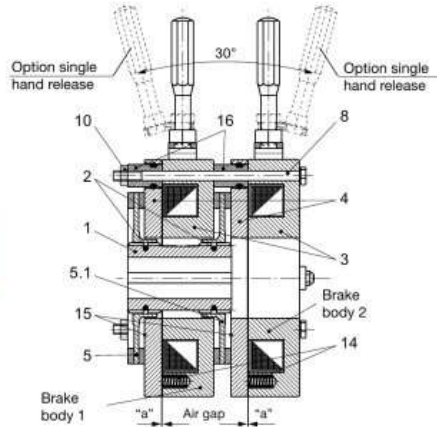
Fig. 2 (Dual circuit brake)
