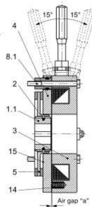
Fig. 3 (Single circuit brake)
