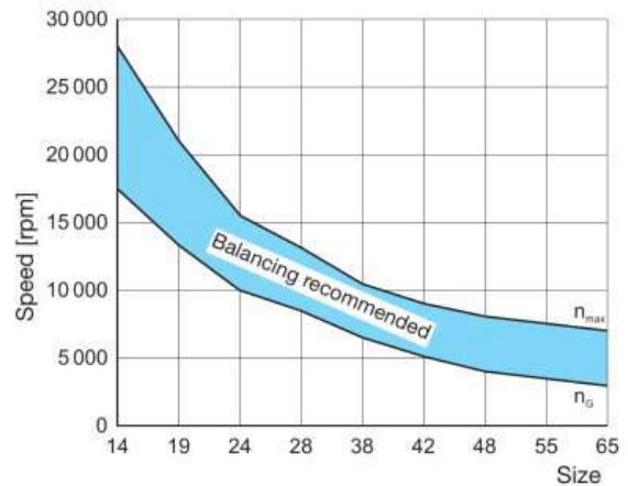
Diagram 1: Balancing the Shrink Disk Hubs
