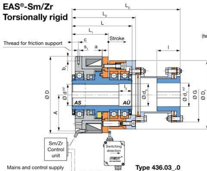
Type 436.03_0
