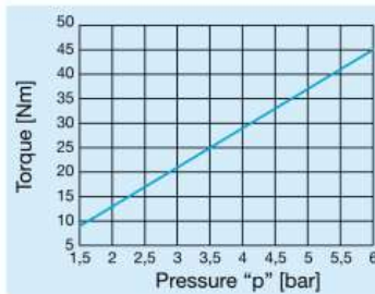
EAS®-Sp 01/450.125.H
