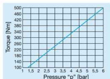
EAS®-Sp 3/45_.125_.
