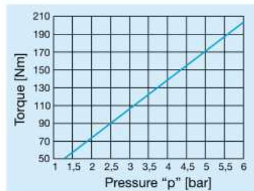
EAS®-Sp 2/45_.125_.
